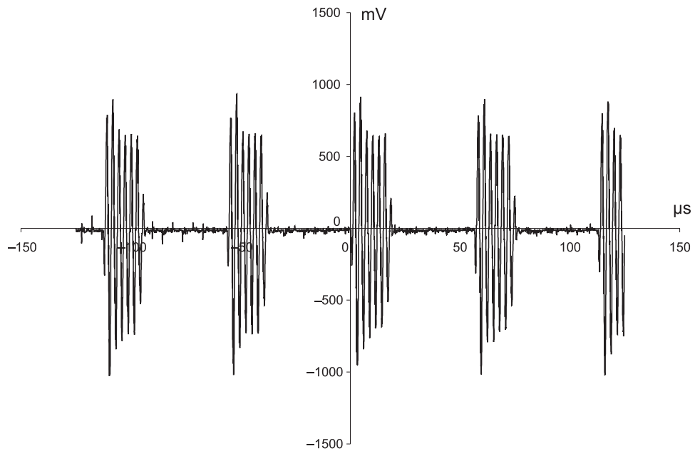
Figure 3. Oscilloscope image of the current in a cable of a surgical diathermy at dry-cut setting. The frequency of the signal is \sim 500 kHz and the repetition frequency for the pulse is \sim 20 kHz.
